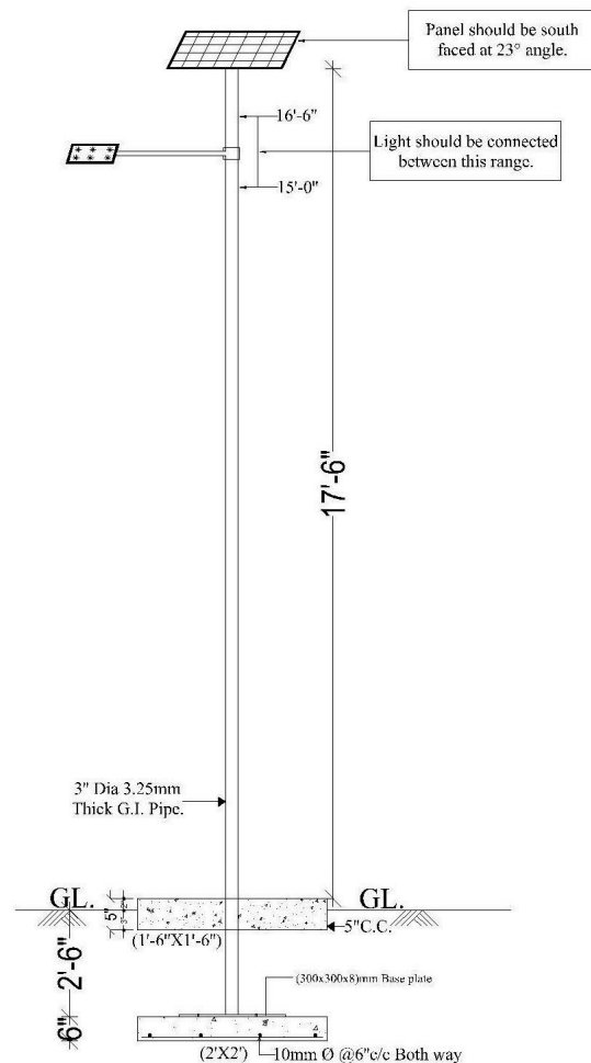
Figure 1: Street Light Design
