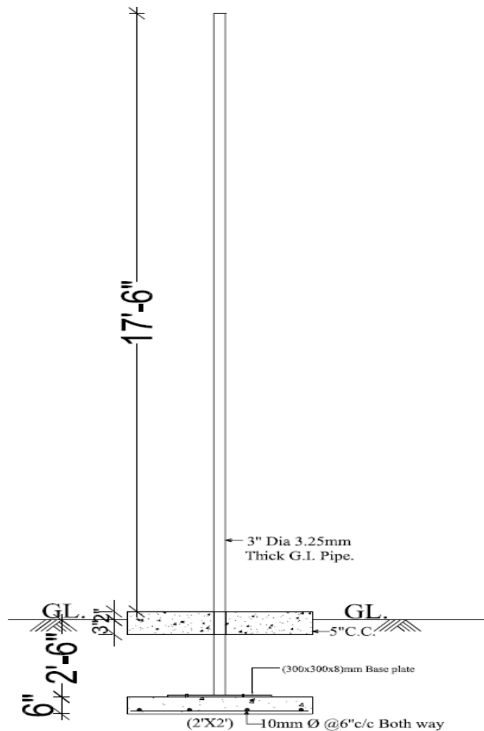
Figure 1: Street Light Design
