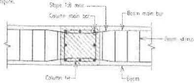
PLAN SECTION OF BEAM COLUMN JOINT
